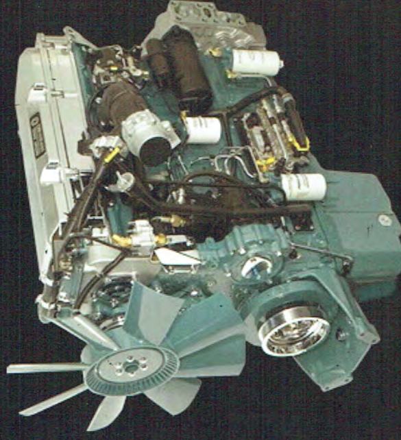
Series 60 EGR & NON EGR Engines
